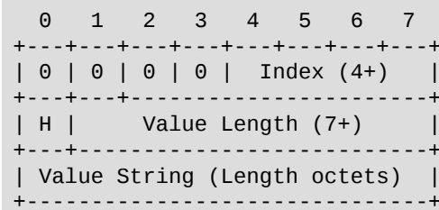
Figure 8: Literal Header Field without Indexing — Indexed Name
