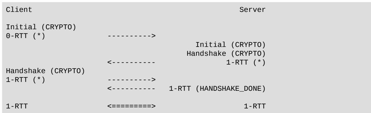
Figure 4: Simplified QUIC Handshake
