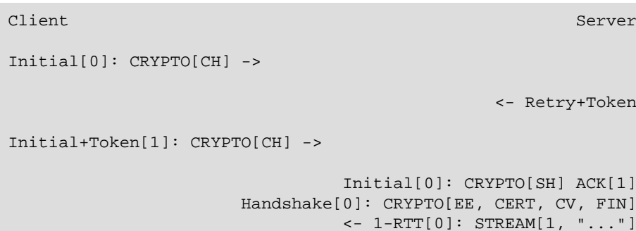
Figure 9: Example Handshake with Retry
